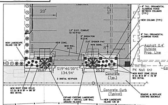
ENTRANCE GATE ENLARGEMENT SCALE: 1"=10'
